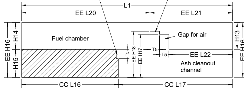
Section E-E
