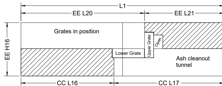
Section E-E With grates in position
